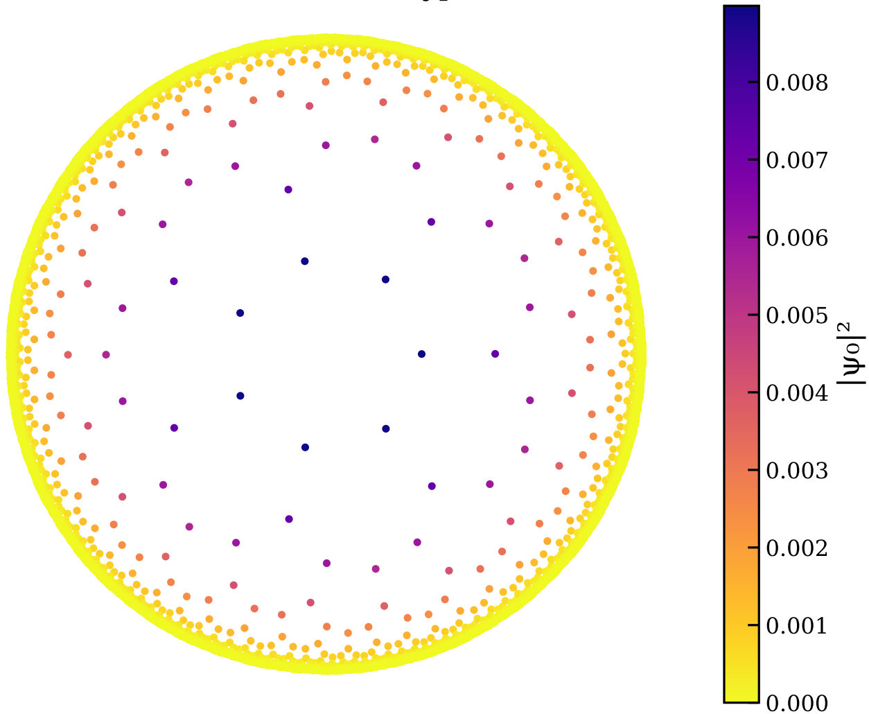
Ground state distribution: Hyperbolic {7,3}
